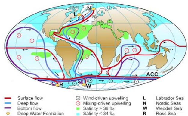
Schematic of the ocean circulation associated with the global Meridional Overturning Circulation (MOC), with special focus on the Atlantic section of the flow (AMOC).
